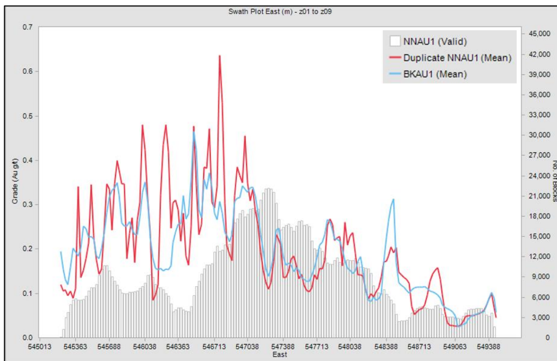
Figure 14-31: Swath plot in Easting – BKAU1 & NNAU1 Estimates
