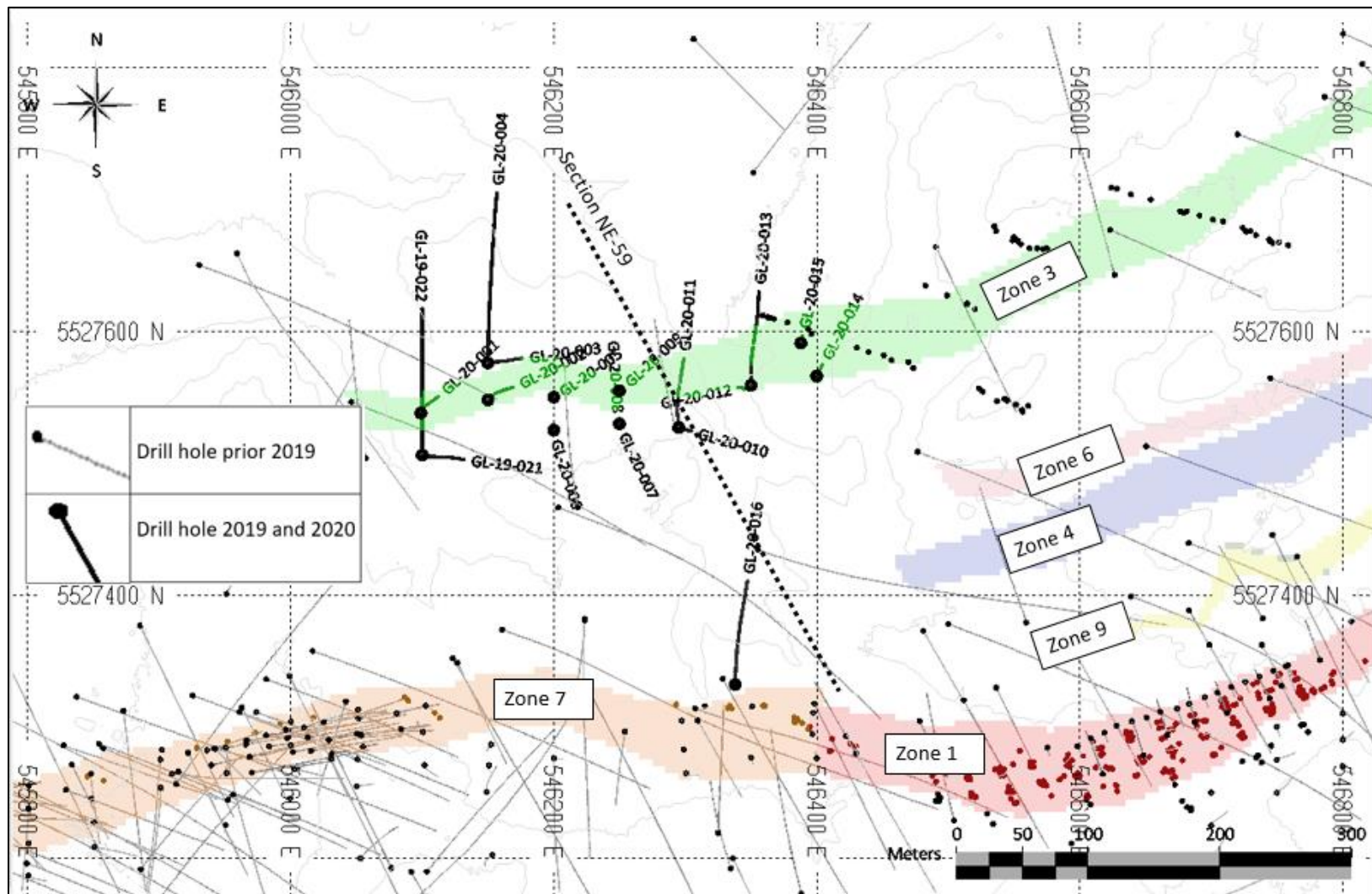
Figure 10-9: Goldlund Drillhole Location Map, 2019-2020, Southwest on Main Zone (Zone 3)
