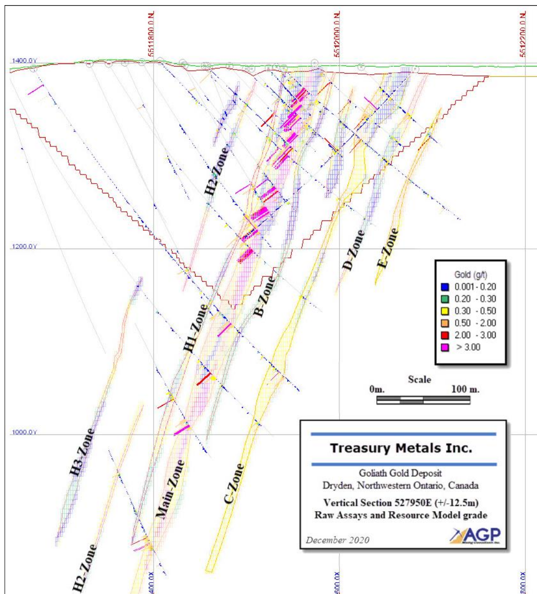
Figure 14-9: Gold Grade Model Distribution
