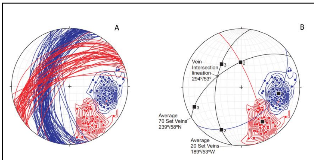
Figure 7-10: Stereonets of the Planes & Poles to Gold-Bearing Veins
