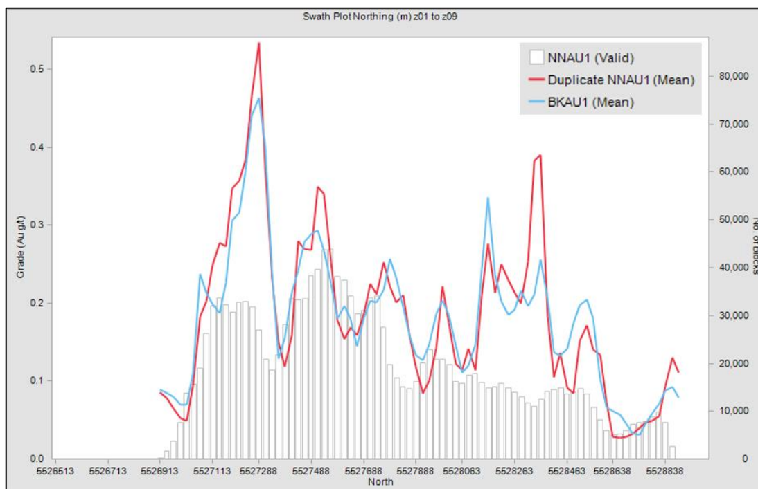
Figure 14-32: Swath plot in Northing – BKAU1 & NNAU1 Estimates
