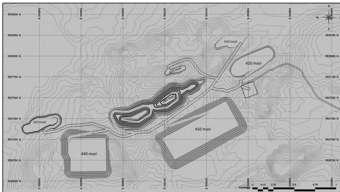
Figure 16-50: End of Year 4 – Goldlund
