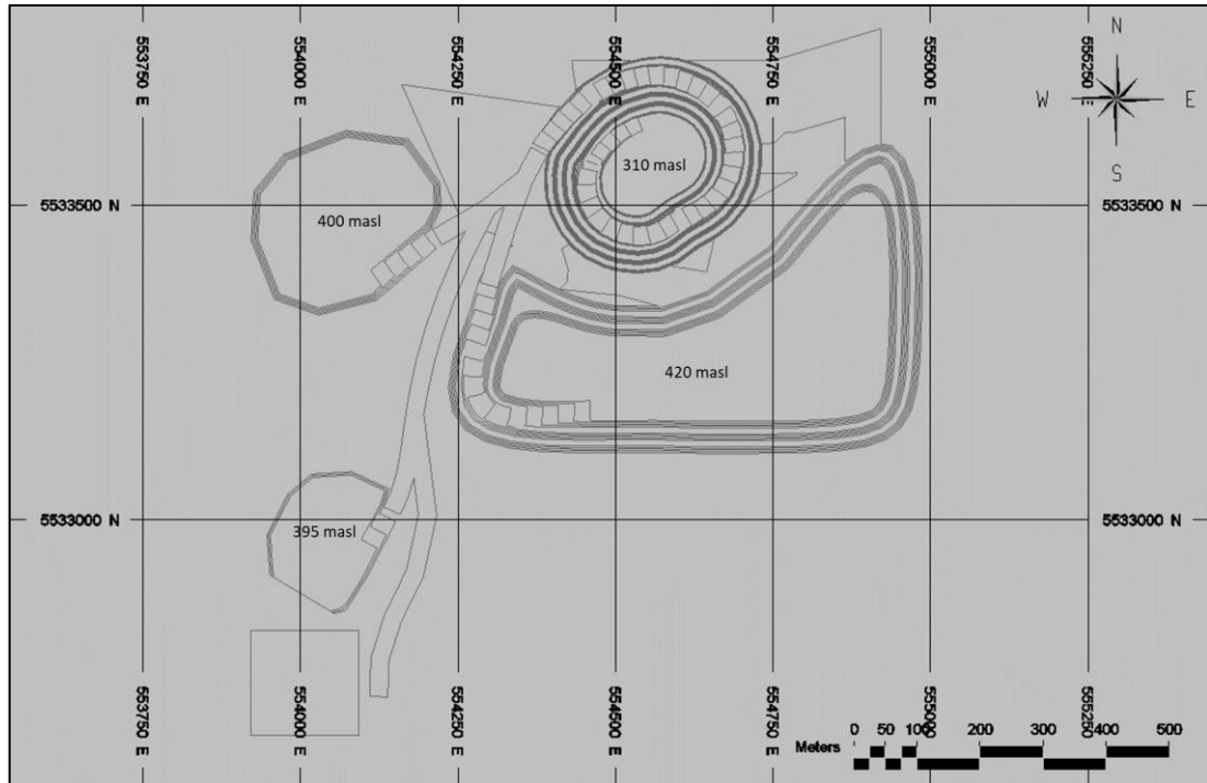
Figure 16-63: End of Year 8 – Miller
