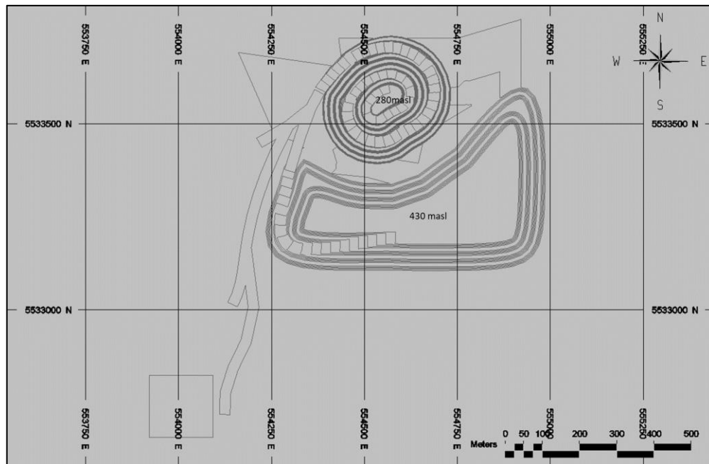
Figure 16-69: End of Year 10 – Miller
