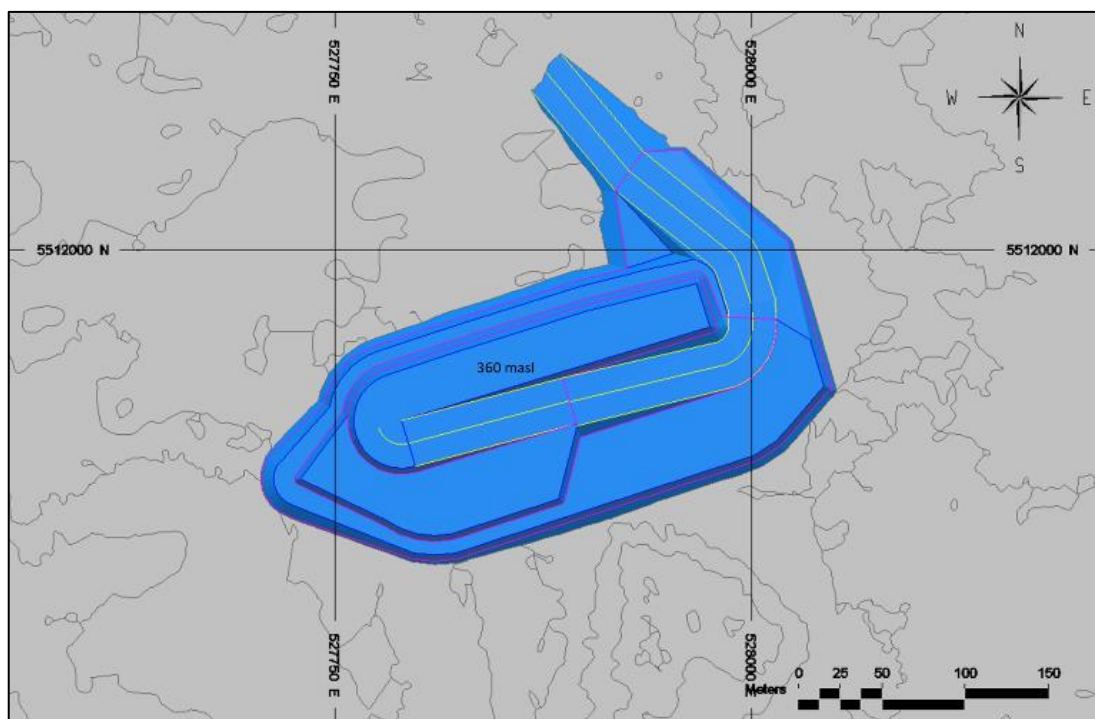
Figure 16-4: Phase 1A Design – Goliath
