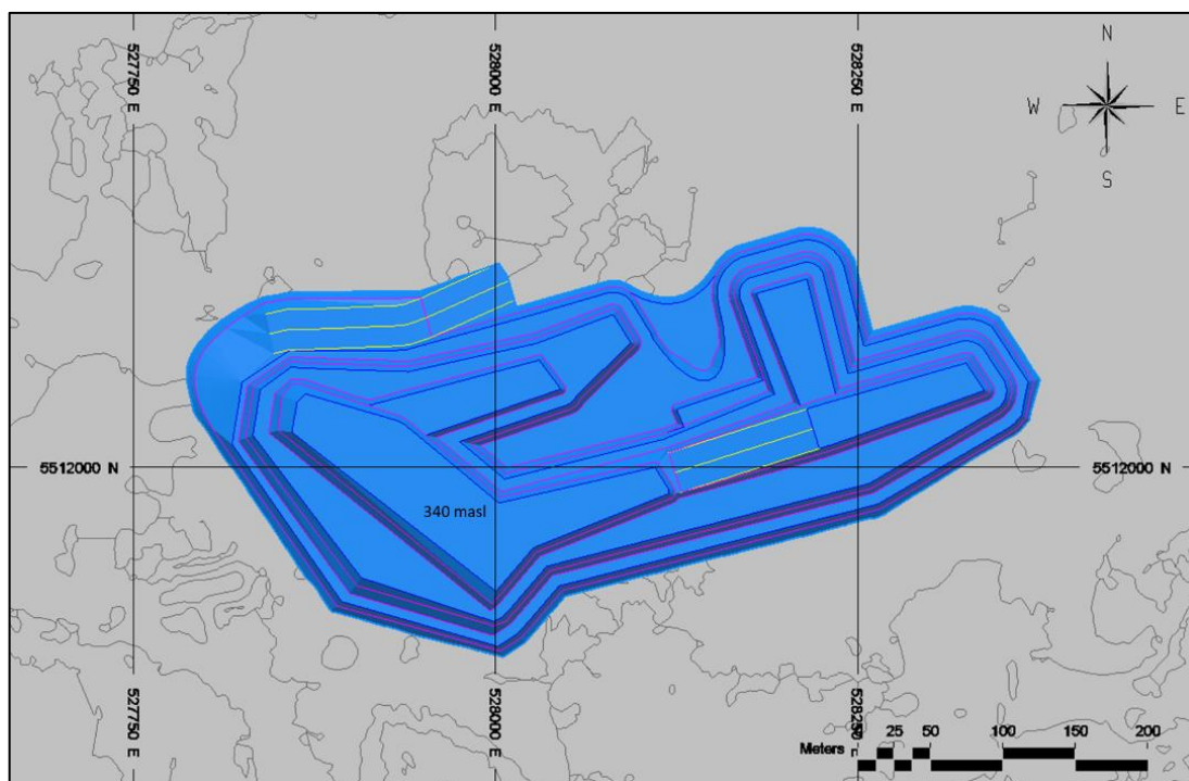
Figure 16-7: Phase 3 Design – Goliath
