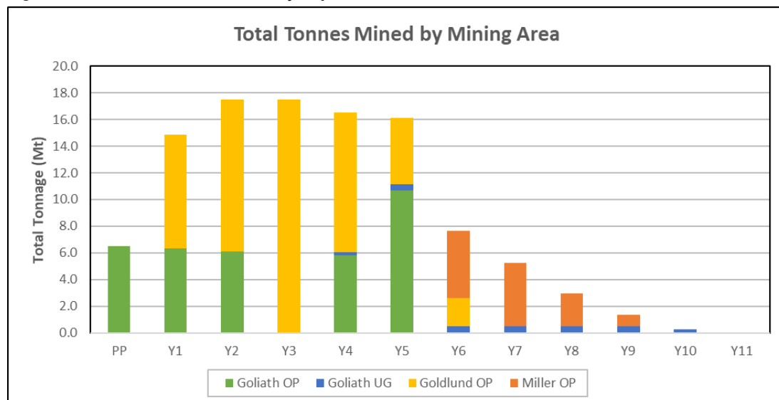
Figure 16-38: Total Tonnes Mined by Deposit
