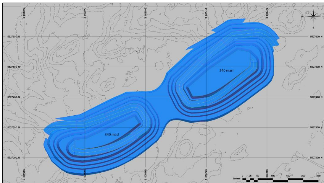
Figure 16-10: Phase 1 Design – Goldlund
