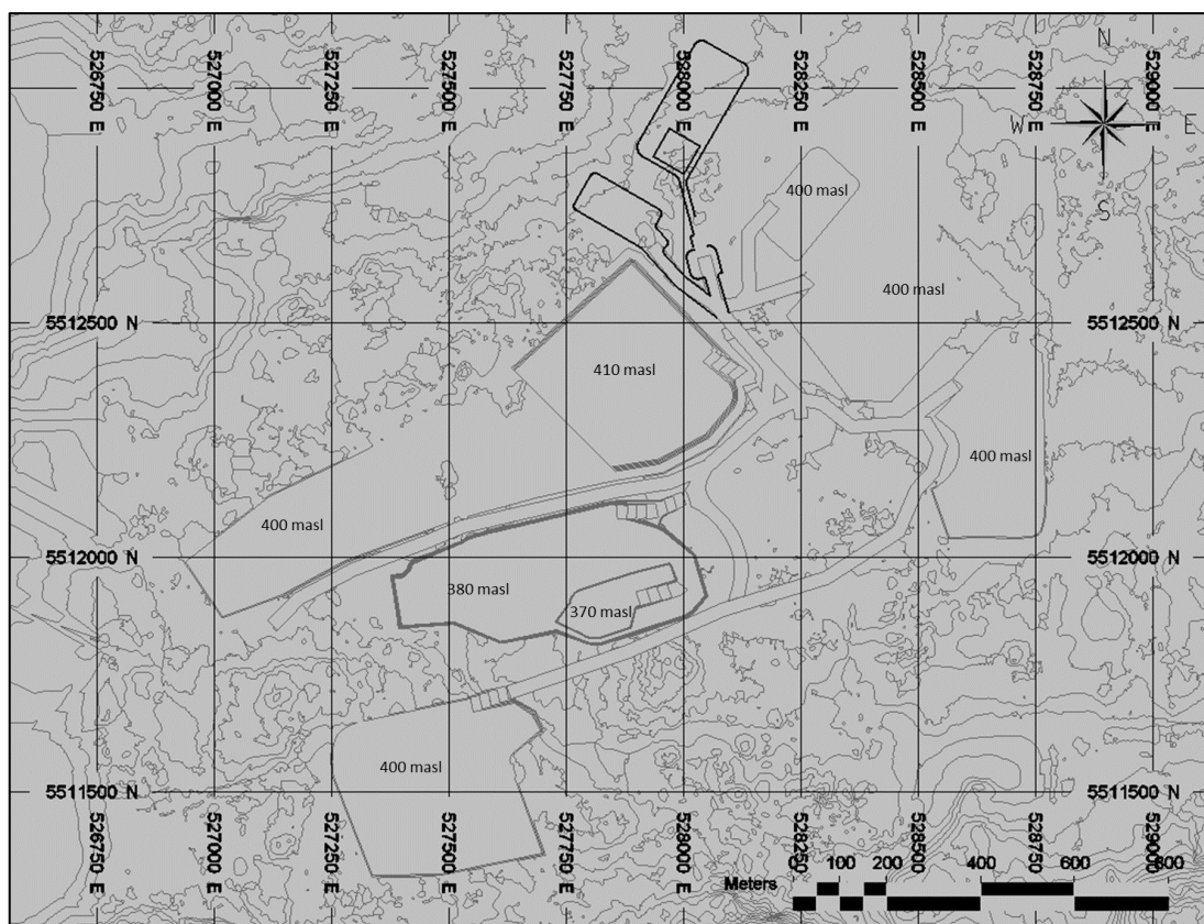
Figure 16-39: End of Pre-Production – Goliath
