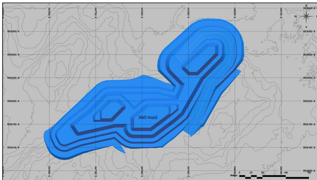
Figure 16-13: Phase 4 Design – Goldlund
