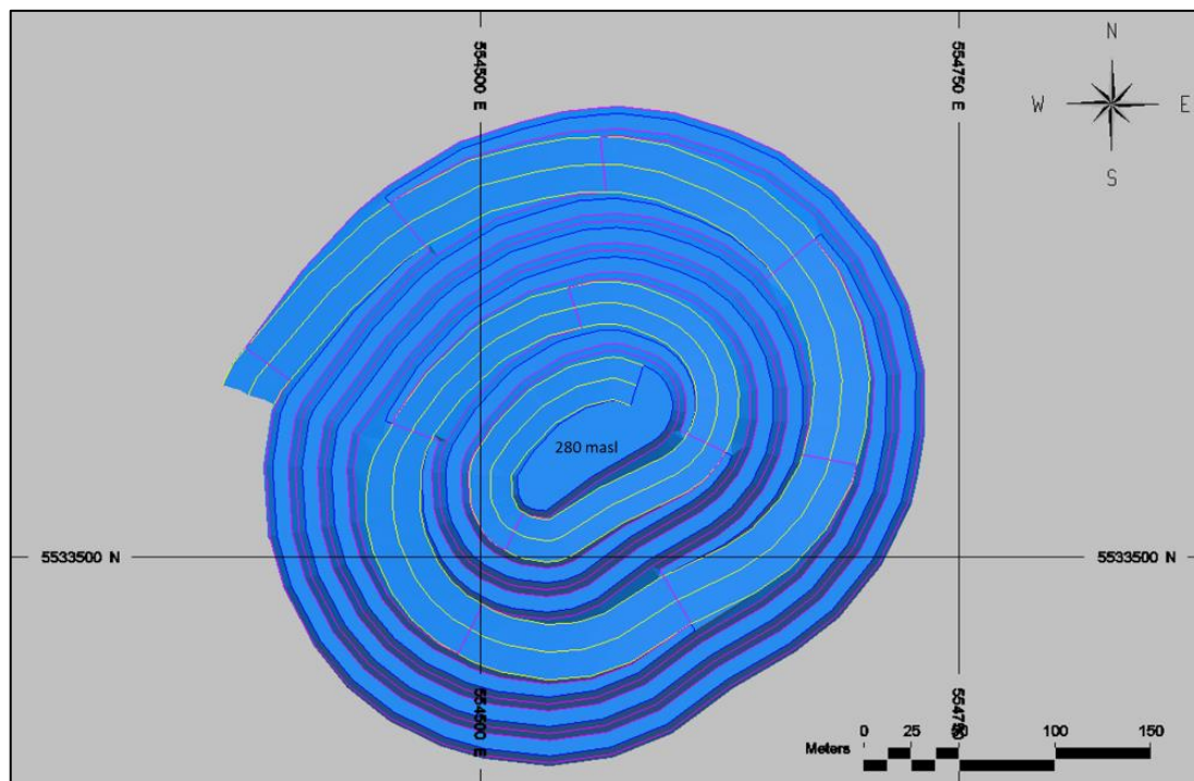
Figure 16-17: Pit Design – Miller
