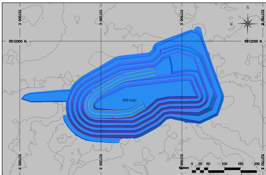
Figure 16-6: Phase 2 Design – Goliath
