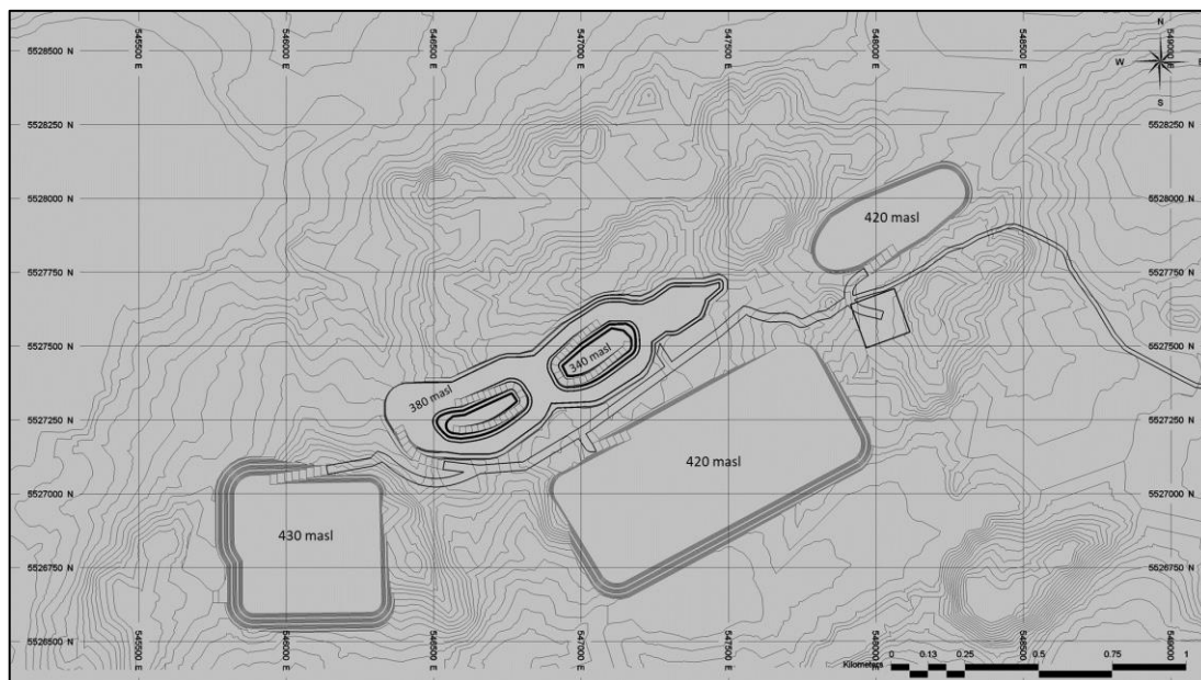
Figure 16-44: End of Year 2 – Goldlund
