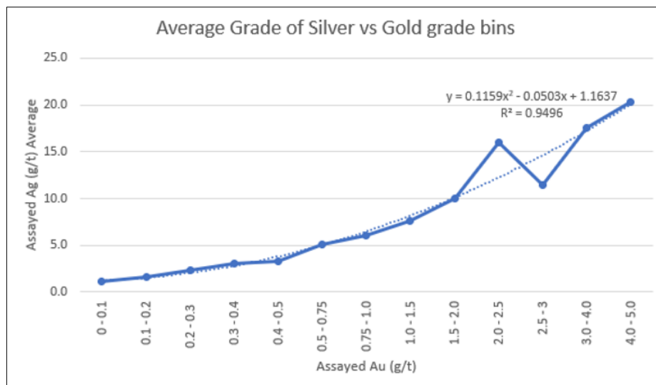
Figure 14-6: Formula to Calculate the Missing Silver Values
