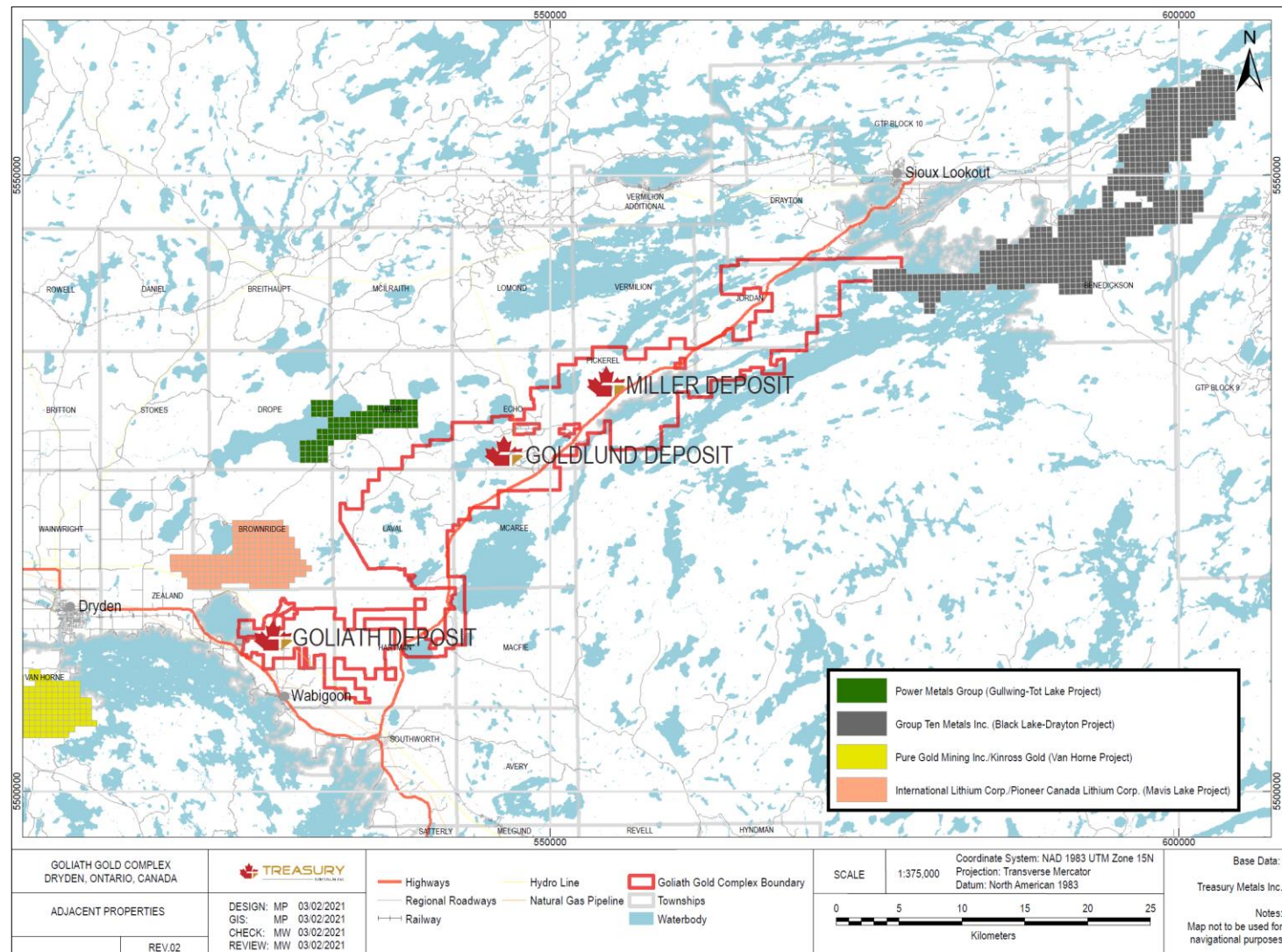
Figure 23-1: Adjacent Properties
