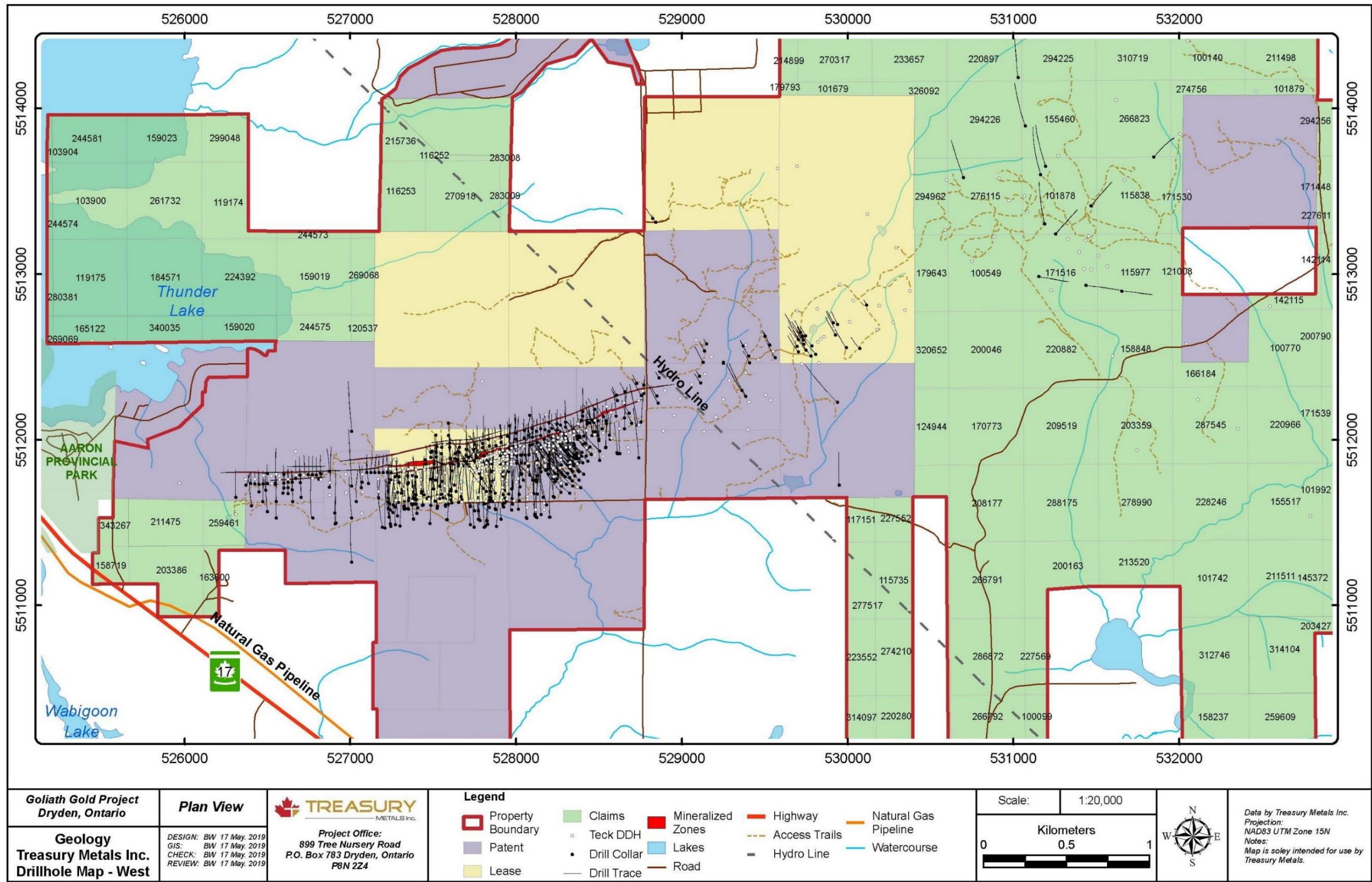
Figure 10-2: Goliath Drillhole Location Map, Treasury Metals, Western Goliath Property
