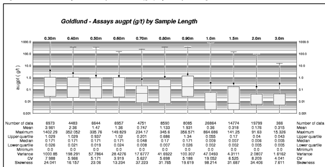
Figure 14-19: Side-by-Side Boxplots of Au (g/t) by Sample Length
