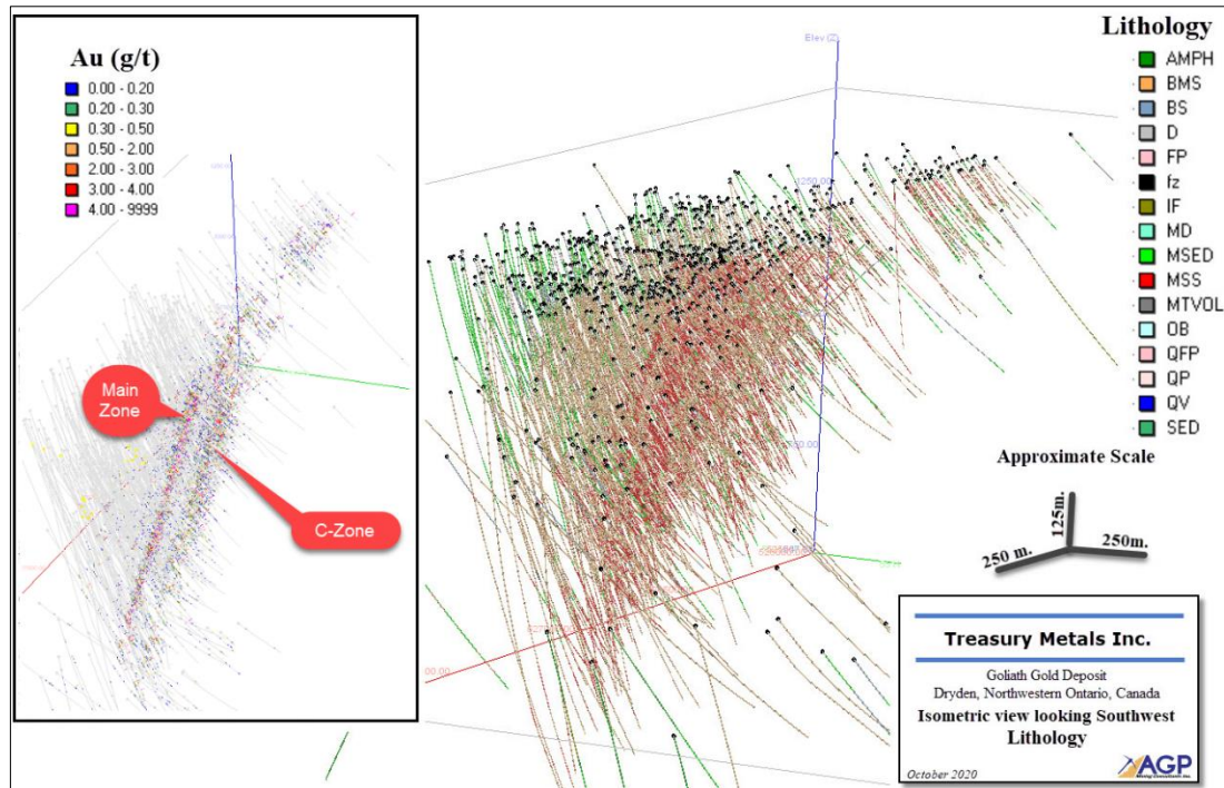
Figure 14-1: Lithology & Assays
