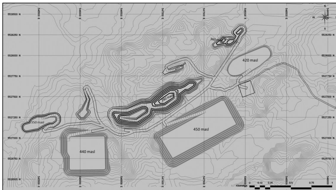
Figure 16-53: End of Year 5 – Goldlund
