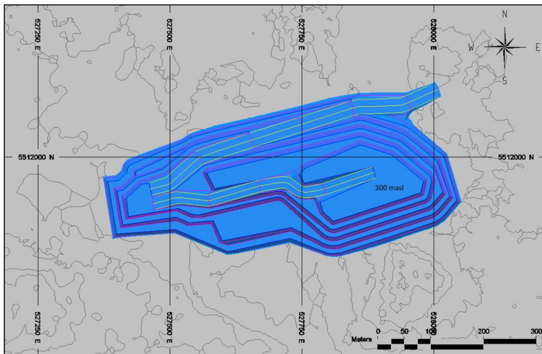
Figure 16-5: Phase 1B Design – Goliath
