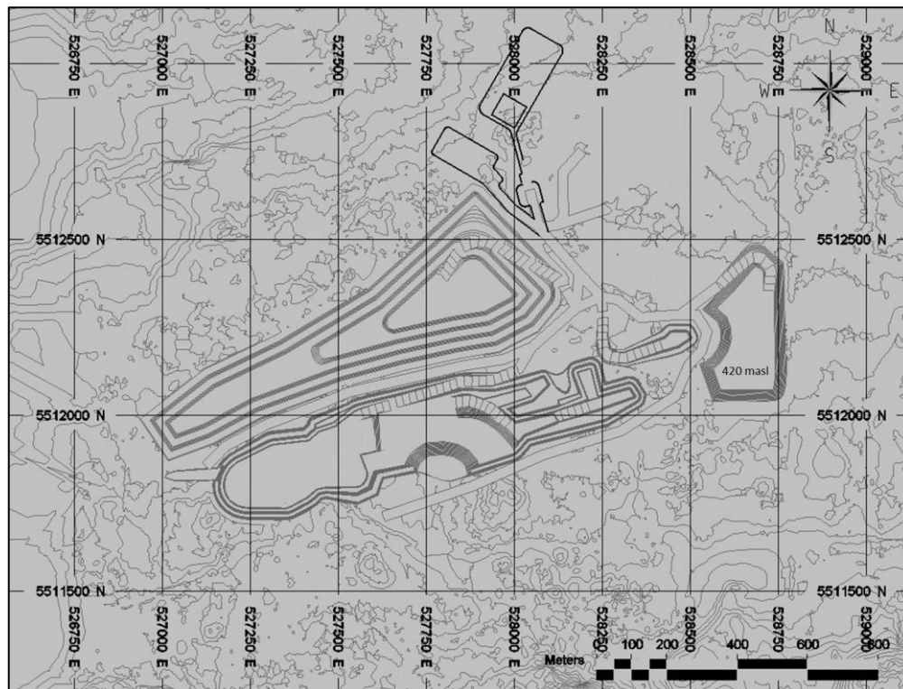
Figure 16-70: End of Year 11 – Goliath Open Pit – Stockpile Rehandle
