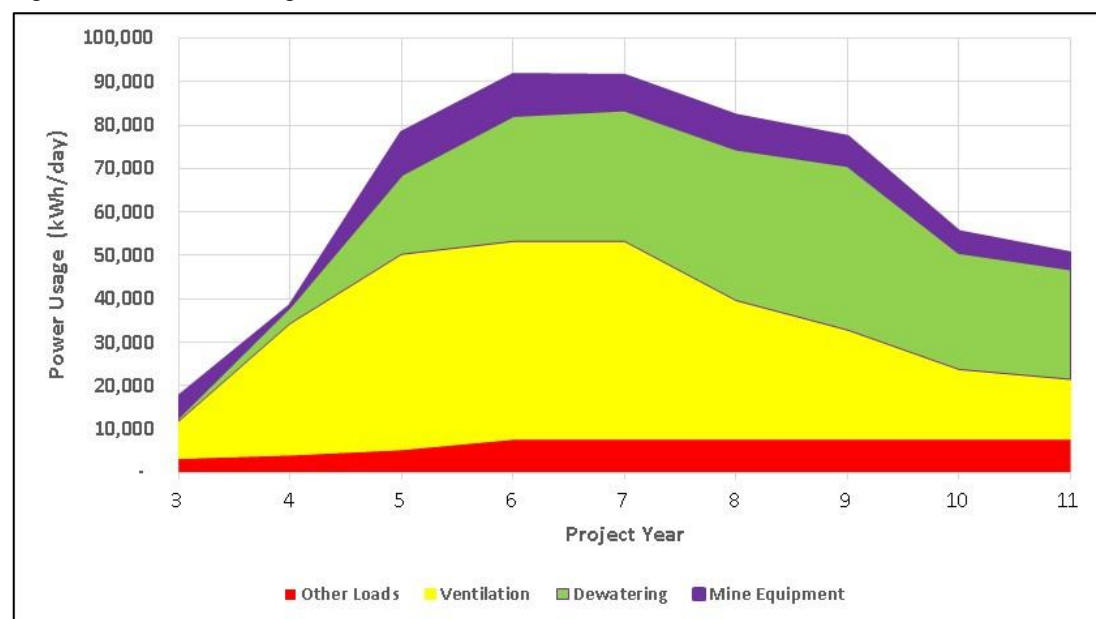
Figure 16-36: Power Usage
