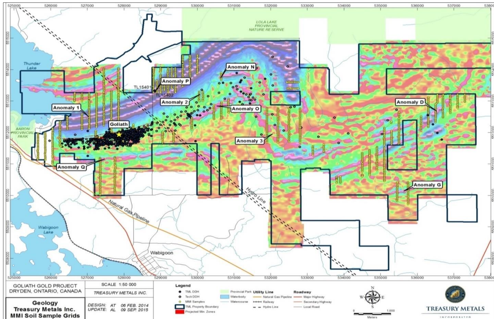
Figure 9-9: 2014 MMI Sample Grid Location Map
