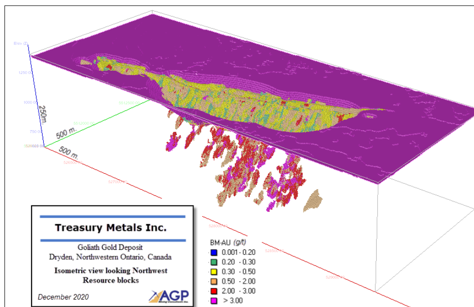
Figure 14-16: Resource Blocks
