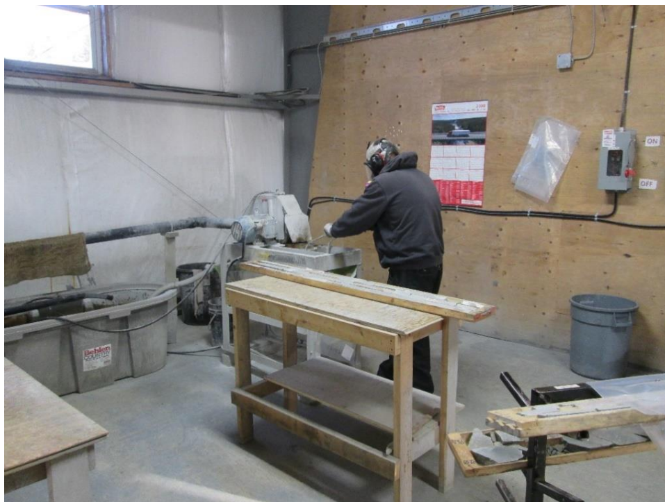
Figure 12-19: Drill Core Sample Saw
