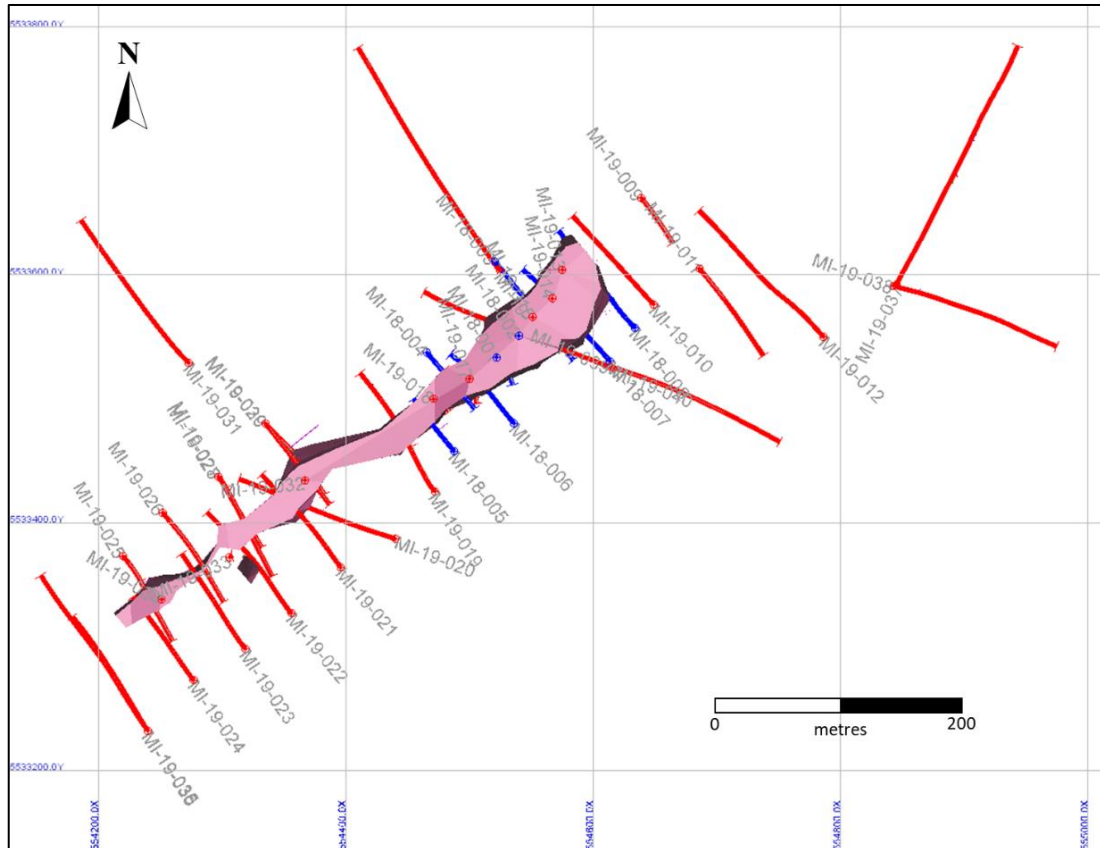
Figure 10-11: Miller Drillhole Location Map
