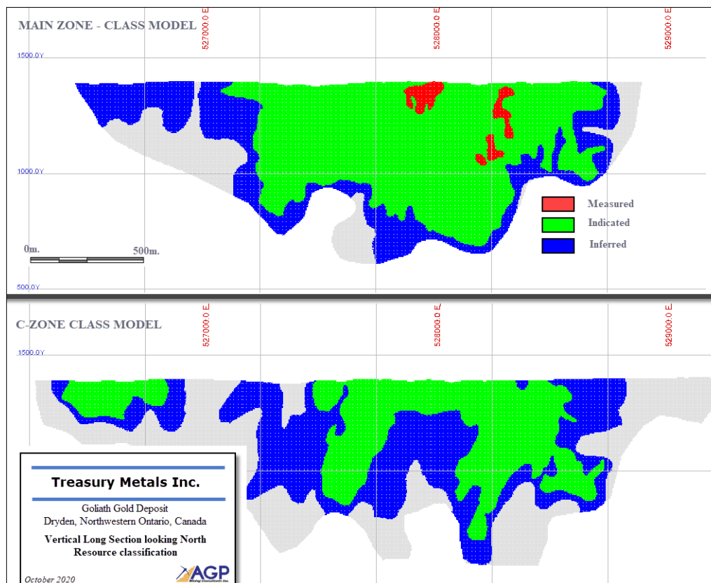
Figure 14-15: Model Classification
