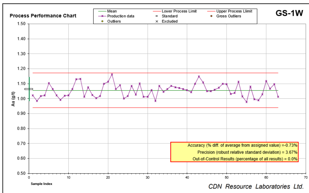
Figure 11-4: Control Chart of GS-1W Standard Results for the 2019-2020 Samples
