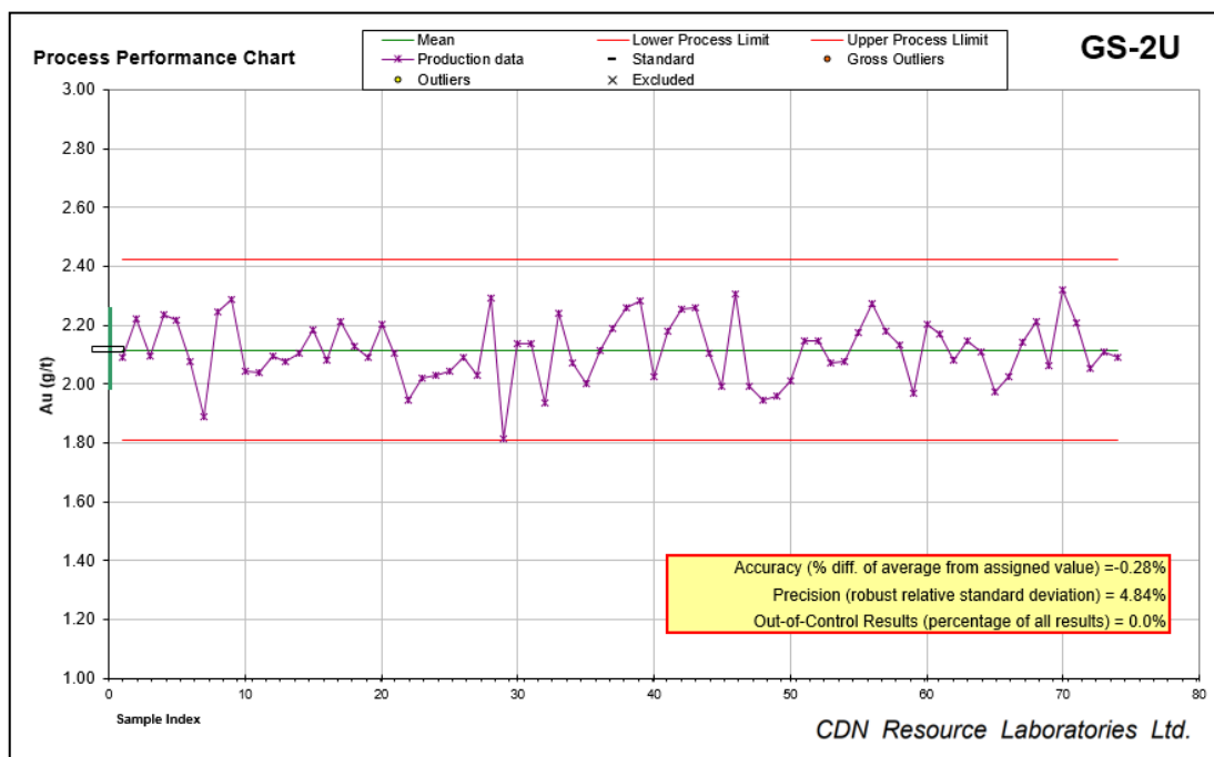
Figure 11-5: Control Chart of GS-2U Standard Results for the 2019-2020 Samples
